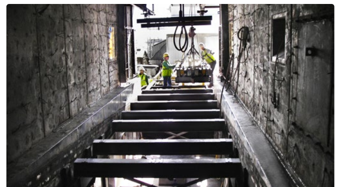
Installation of FLSmidth Cross-Bar cooler inside existing cooler housing
